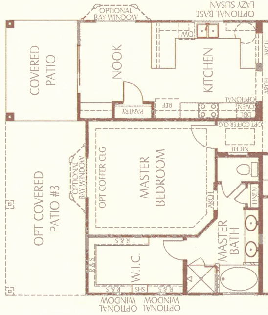
OPTIONAL KITCHEN
